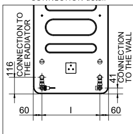
CONNECTION detail
