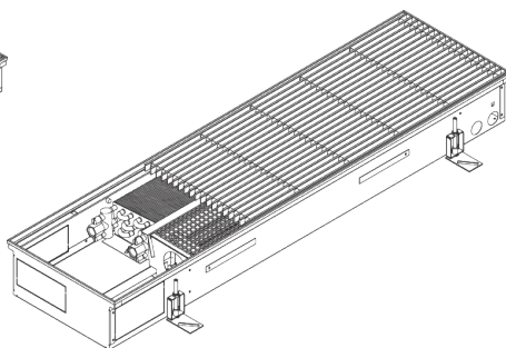
2-Rohr-System
